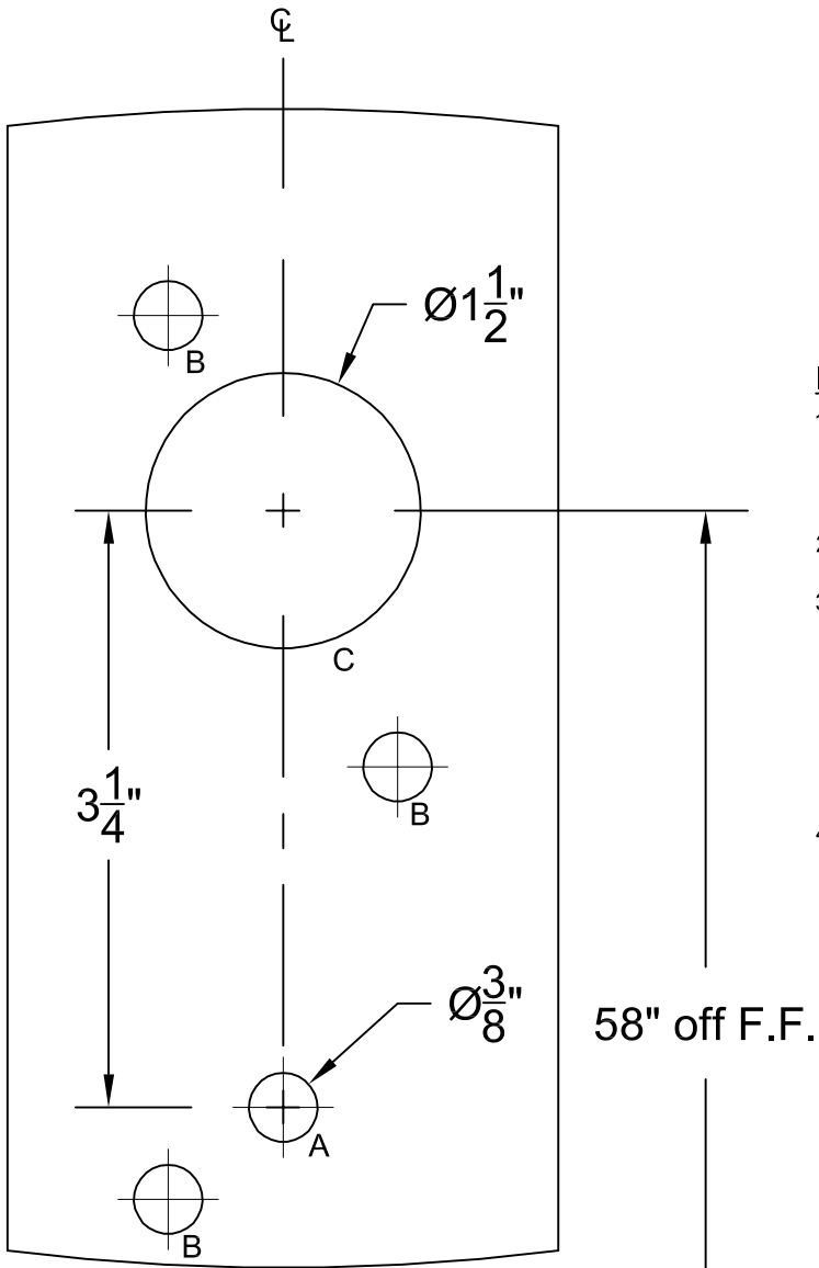
CHIME BASE INSIDE OF DOOR
